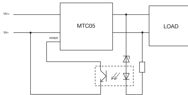
Figure 15. Overshoot Protection - Trip & Restart
