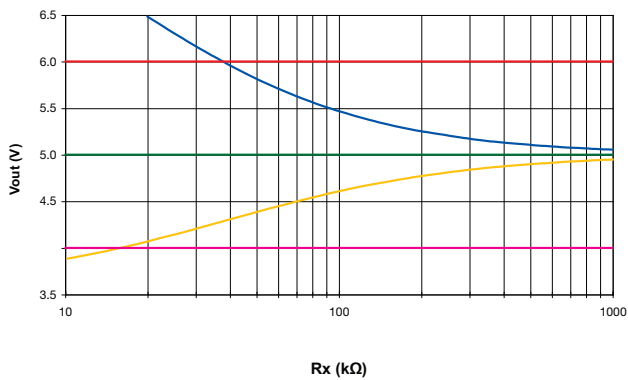
Figure 5. MTC3028S05 - Max and Min Adjustment
