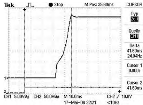
Figure 20. Start up time for MTC1528S28 at full load and 150 \mu F - 41.6 ms
