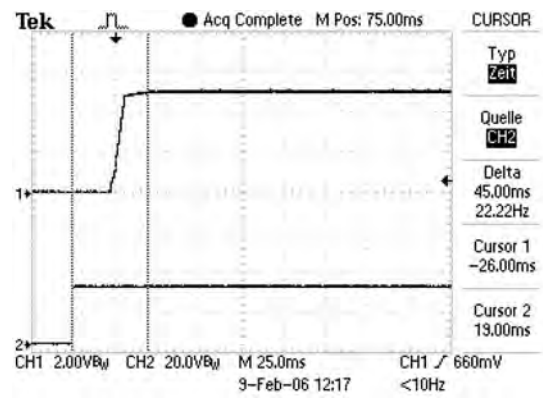
Figure 18. Start up time for MTC3028S05 at full load and 1500 µF - 45 ms
