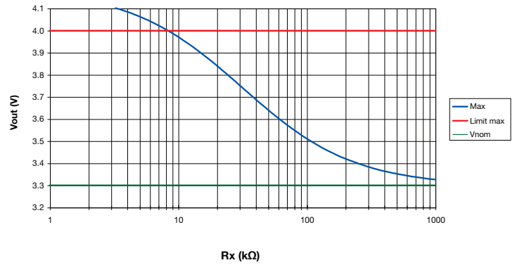
Figure 4. MTC1528S3V3 - Max and Min Adjustment
