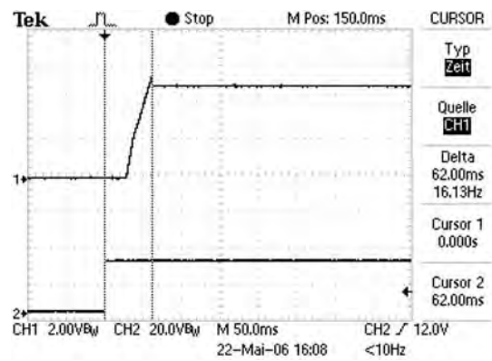
Figure 18. Start up time for MTC0528S05 at full load and 240 µF - 62 ms
