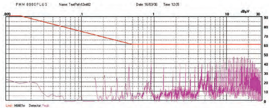
Figure 10. MTC3028S12 with MTF50 filter
