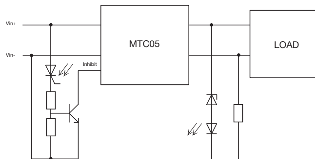
Figure 14. Overshoot Protection - Latched
