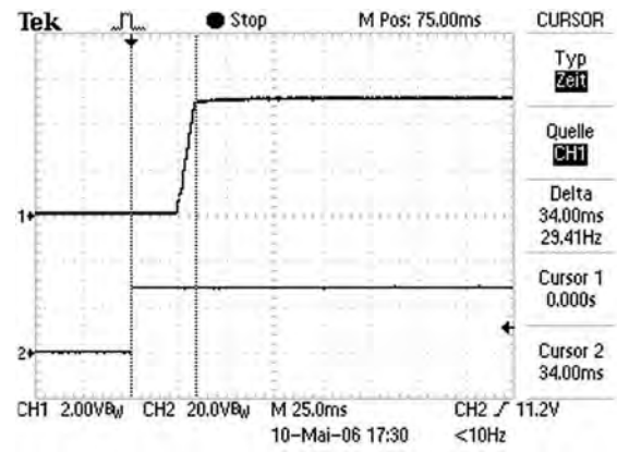
Figure 18. Start up time for MTC1528S05 at full load and 790 \mu F - 34 ms
