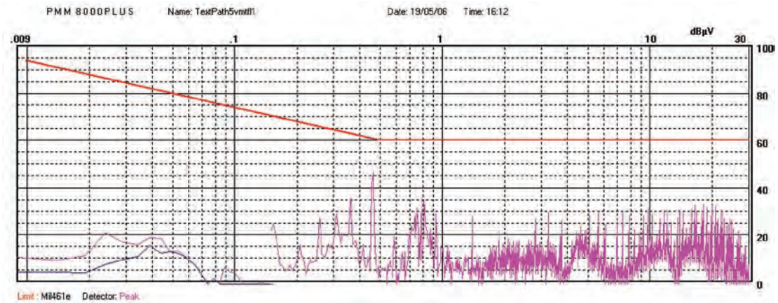
Figure 10. MTC1528S05 with MTF50 filter
