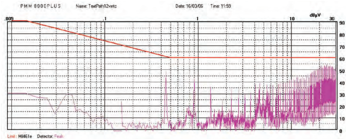
Figure 9. MTC3028S12 without a filter
