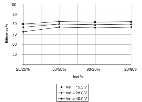
Figure 16. Typical efficiency for MTC3028D15
