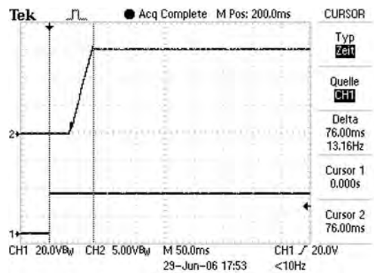
Figure 20. Start up time for MTC0528S28 at full load and 99 µF - 76 ms
