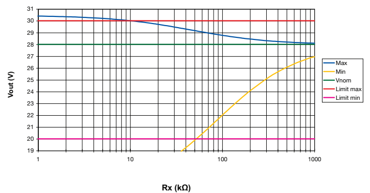
Figure 8. MTC3028S28 - Max and Min Adjustment
