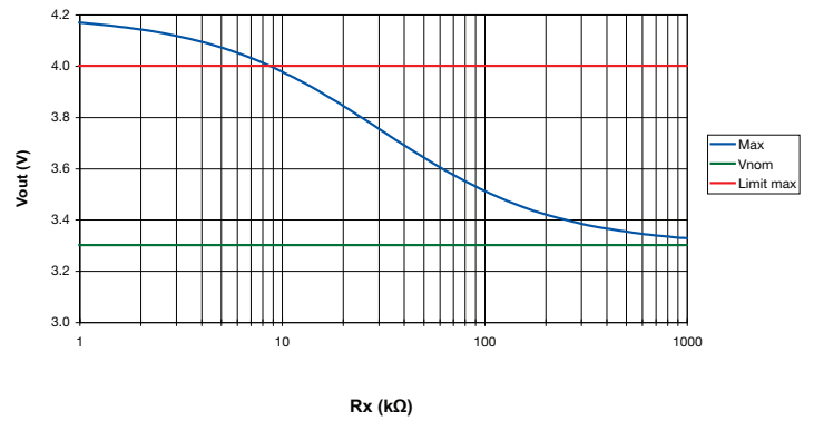
Figure 4. MTC3028S3V3 - Max and Min Adjustment
