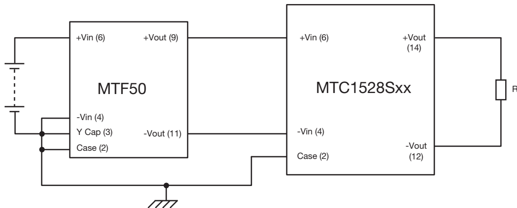
Figure 11. MTC15 - EMC Filter connection diagram
