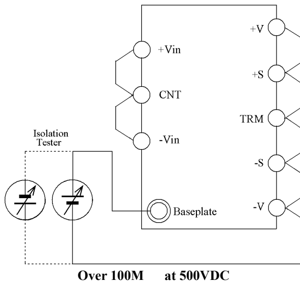
Fig.20-1 Isolation Test
