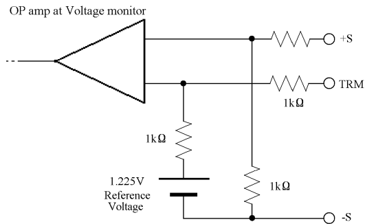
Fig.2-7 Internal TRM Circuit (For the Reference)
